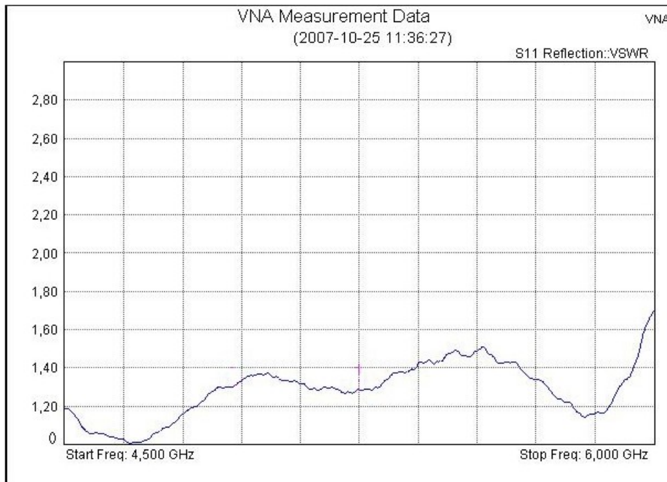
Panel antenna 5GHz
